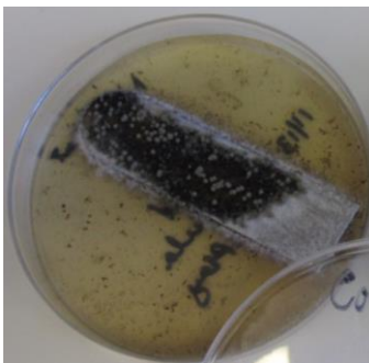
Fig3: Positive control - heavy fungal growth © Accugen labs
