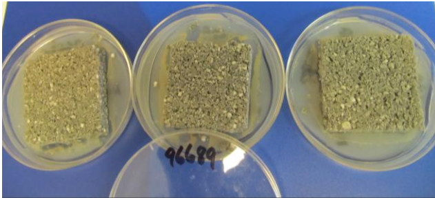
Fig1: Lab# 96689 at Nutrient Salt agar inoculated with fungal spores at 28 days in triplicate Test sample did not support any fungal growth. © Accugen labs
